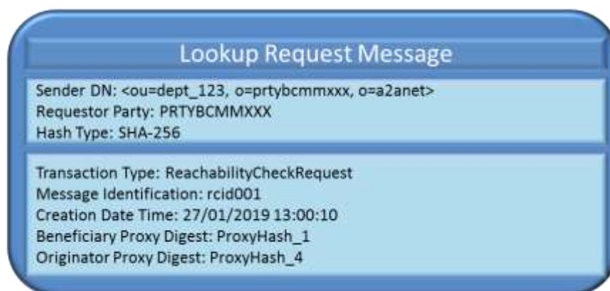
Figure 12 – Successful scenario 1 – Reachability Check Request
