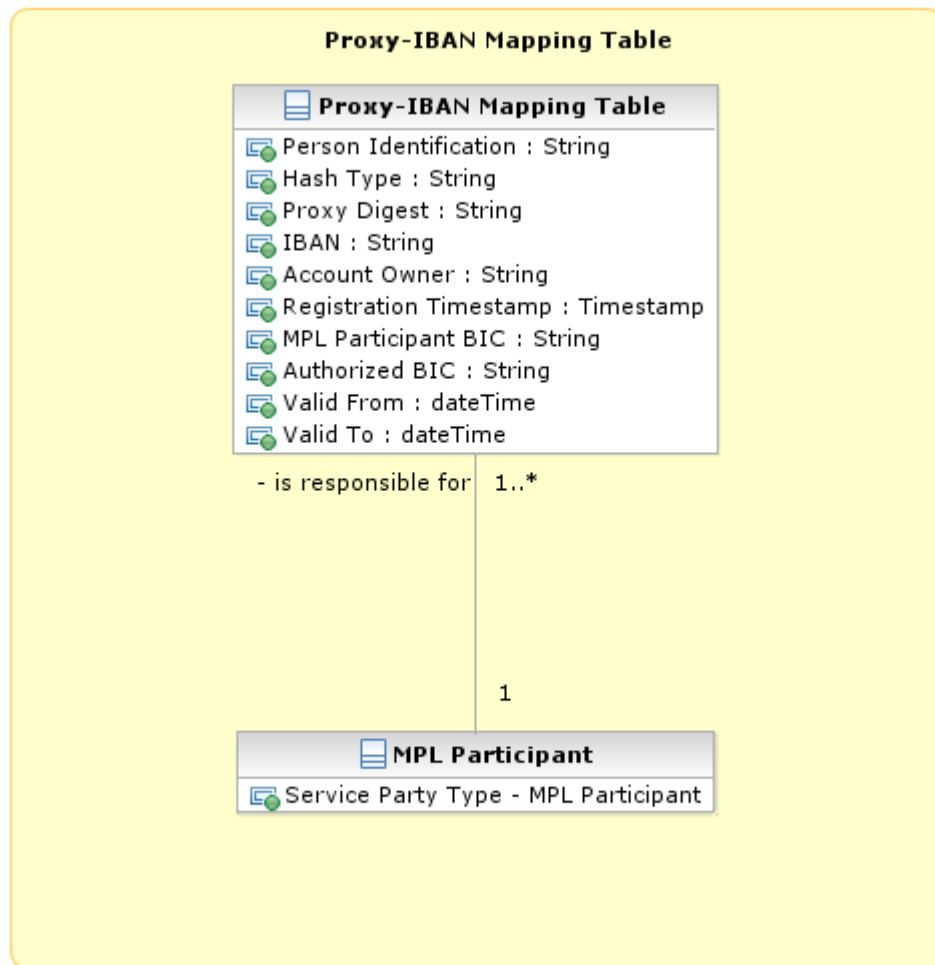
Figure 2 – Proxy-IBAN Mapping Table
