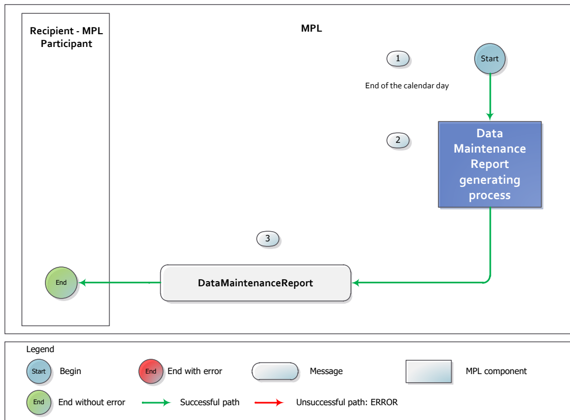
Figure 59 – MPL Repository Maintenance Report flow
