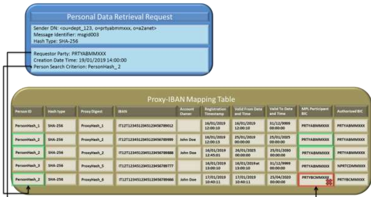
Figure 55 – Successful scenario 3 – PersonalDataRetrievalRequest
